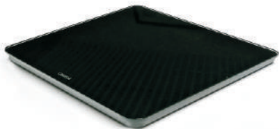
PCF048-10 Weight Scale Size:290x290x30mm Weighing scope:3.0-200kg Display:Led white light Power supply:Three AA batteries
